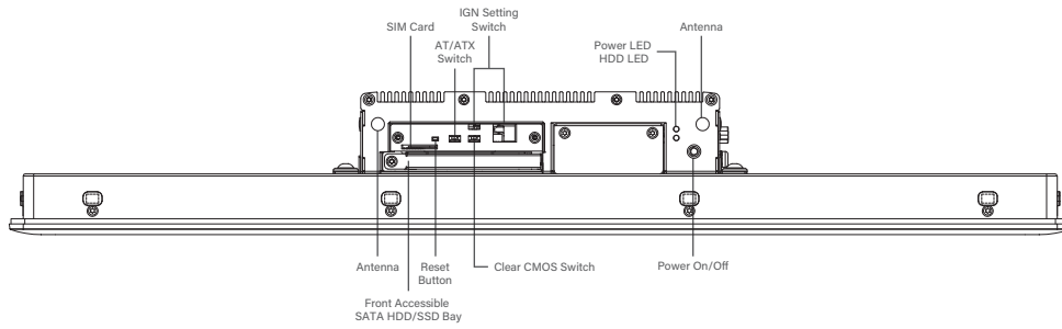
Front I/O
