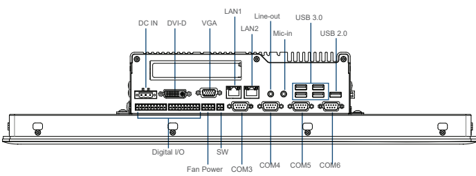
Front I/O
