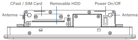
Front I/O
