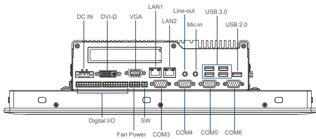
Front I/O
