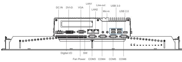
Front I/O
