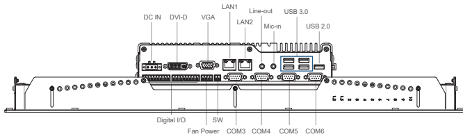
Front I/O
