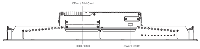
Rear I/O
